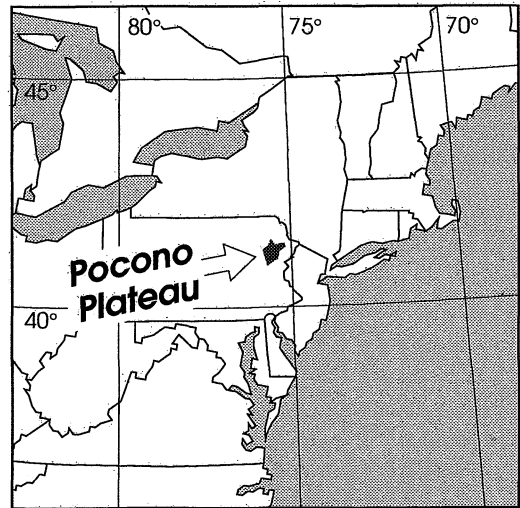
Fig. 1. Location of study area (Pocono Plateau boundary from Berg et al. 1989).
